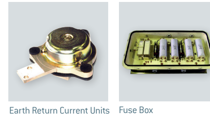
Earth Return Current Units Fuse Box
