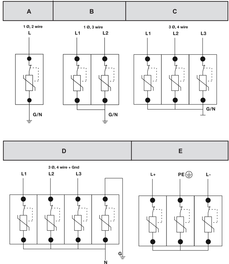
Figure 4 Wiring Diagrams - Modular & Pluggable
