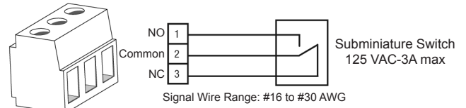
Figure 3 Microswitch
