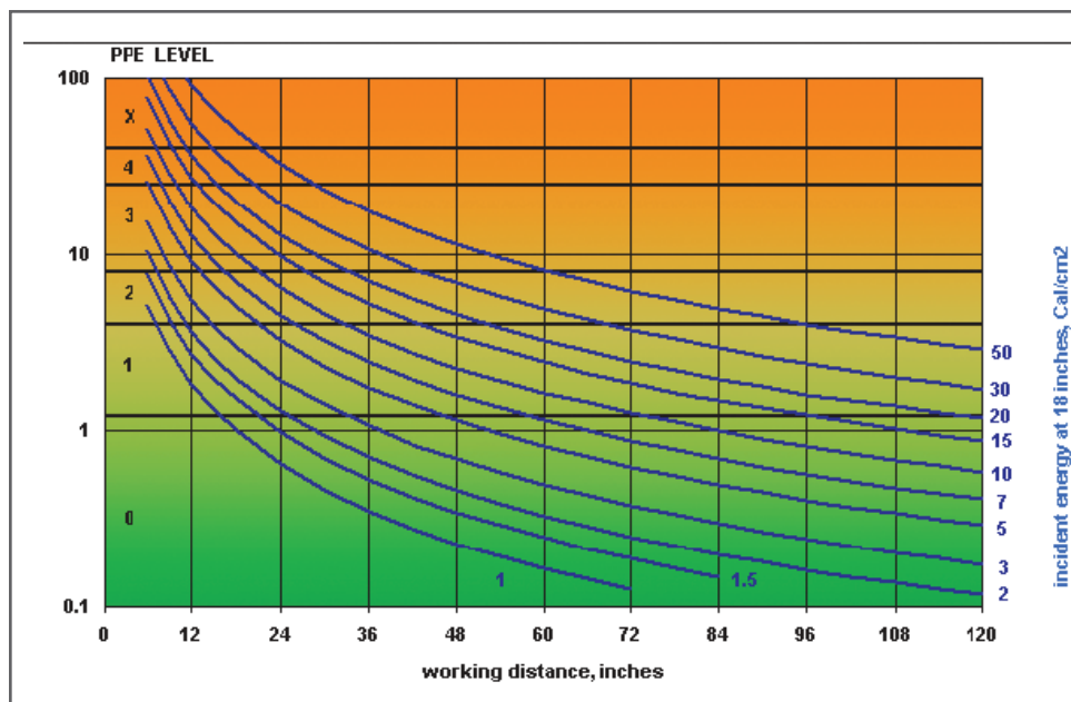
Chart 3: Working Distance Correction Chart
