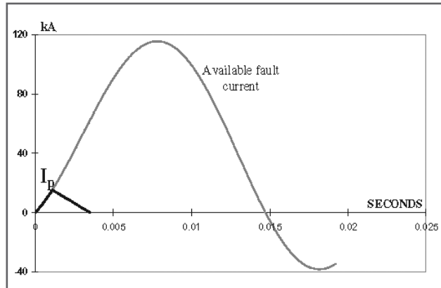
Figure 4: Current Limited Waveform
