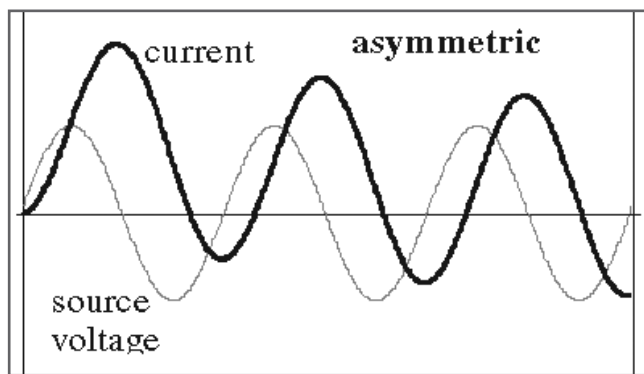
Figure 6: Asymmetrical current waveform
