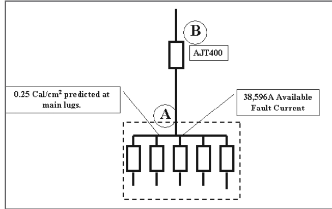
Figure 1: One-line diagram
