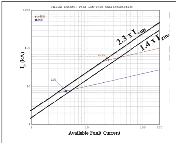
Chart 4: Let through chart
