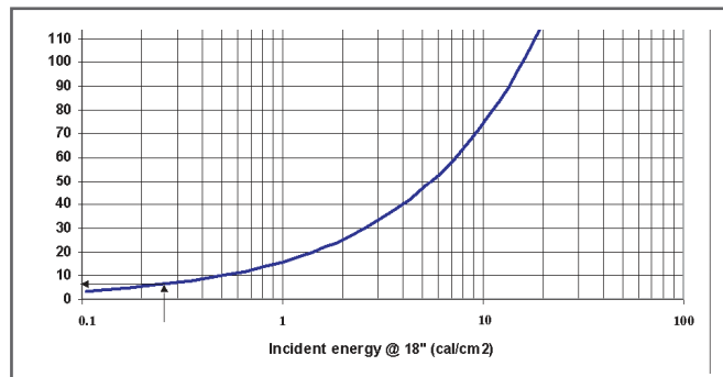
Chart 2: Flash Protection Boundary
