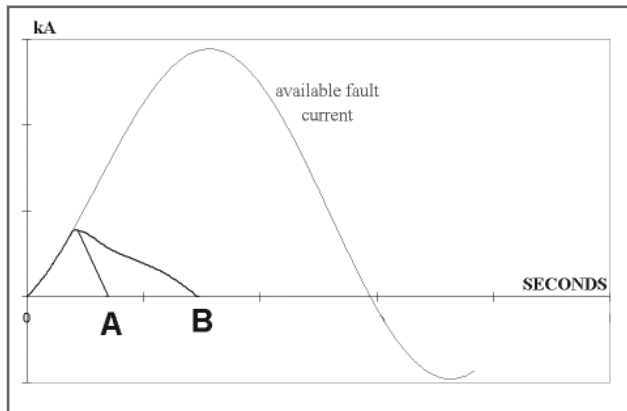
Figure 5: Clearing time effects on I^2t
