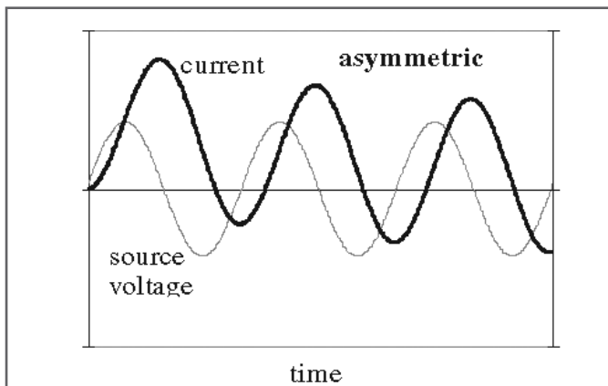
Figure 2: Typical short circuit current waveform
