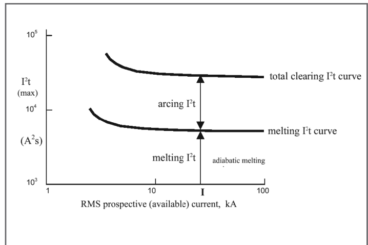
Figure 8: I^2t versus available fault current
