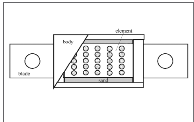
Figure 3: Cut away view of short circuit element
