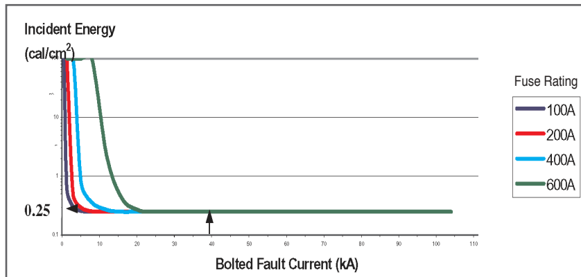
Chart 1: Incident Energy Chart for A6D, AJT and A6T at working distances of 18 inches
