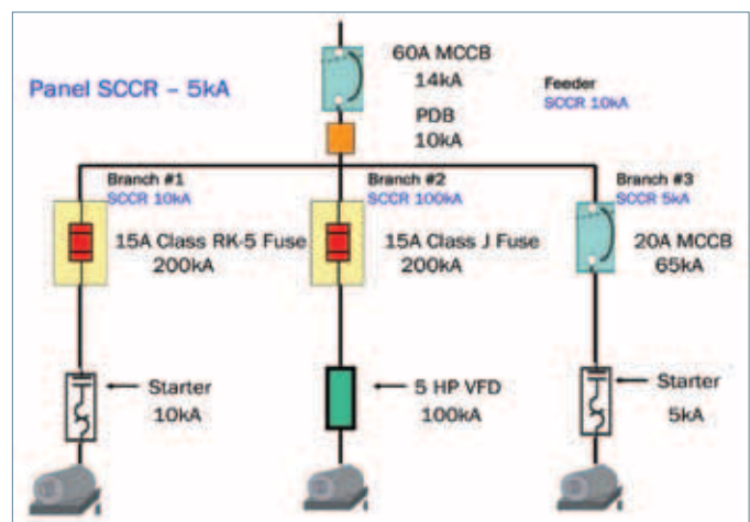
Figure 5: Panel with a low SCCR
