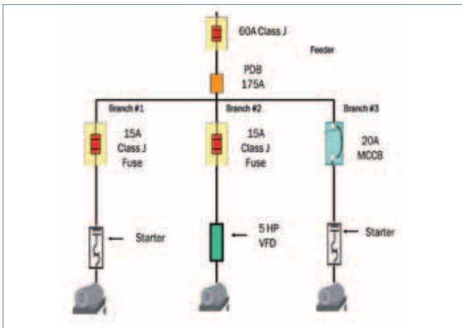
Figure 1: Control Panel
