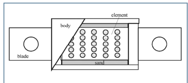
Figure 3: Cut away view of short circuit element
