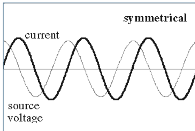
Figure 7: Symmetrical current waveform
