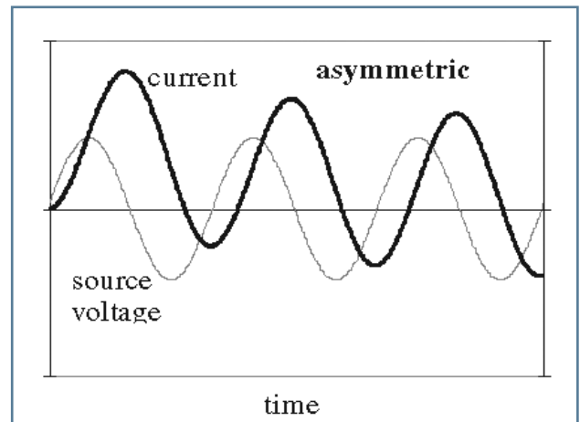
Figure 2: Typical short circuit current waveform
