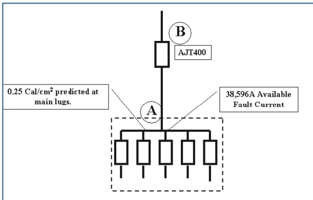
Figure 1: One-line diagram
