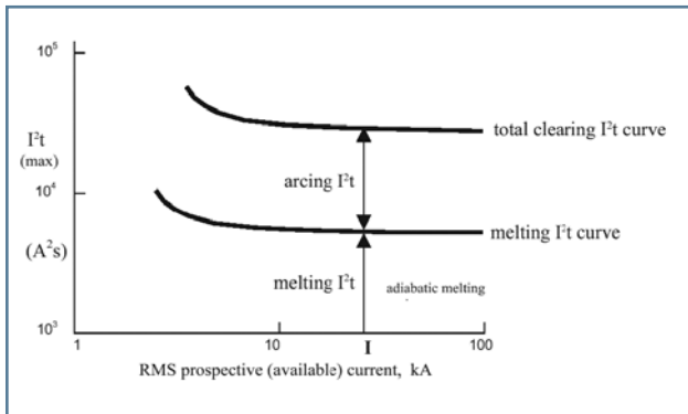
Figure 8: I^2t versus available fault current
