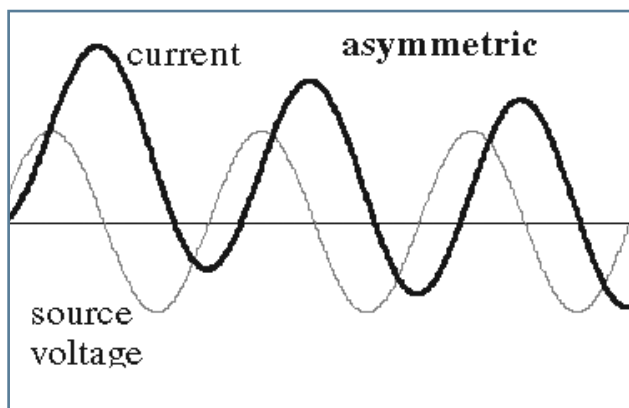
Figure 6: Asymmetrical current waveform
