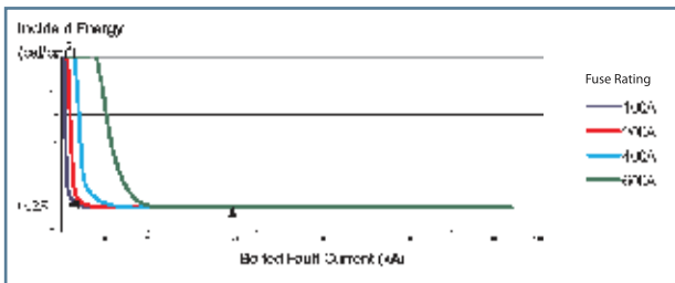
Chart 1: Incident Energy Chart for A6D, AJT and A6T at working distances of 18 inches
