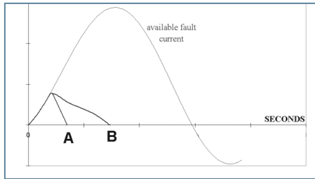
Figure 5: Clearing time effects on I^2t
