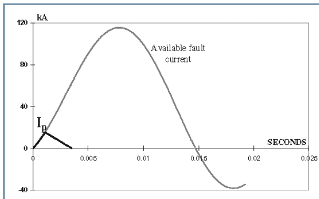
Figure 4: Current Limited Waveform
