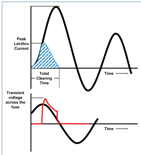
Figure 3. Current-limiting performance.
