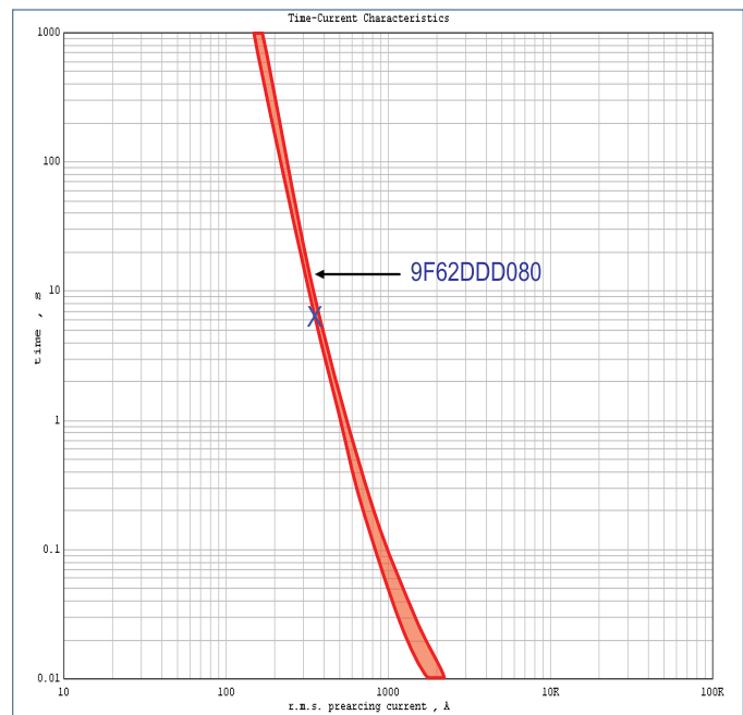
Figure 2: Time current curve for primary fuse.
