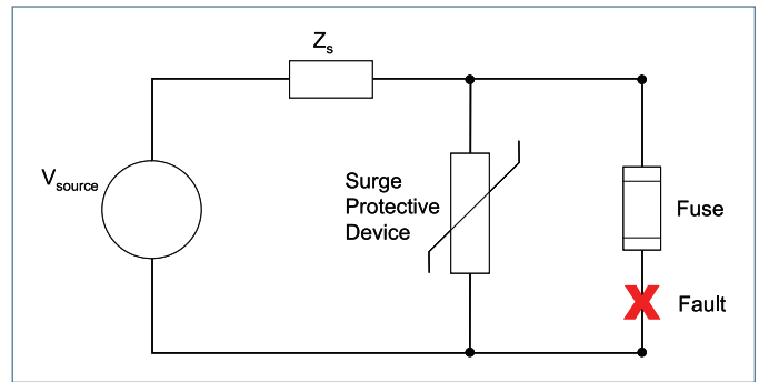
Figure 4. Circuit for transient voltage.
