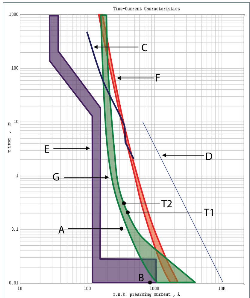
Figure 7 Time Current Curve evaluation for replacement fuse.
