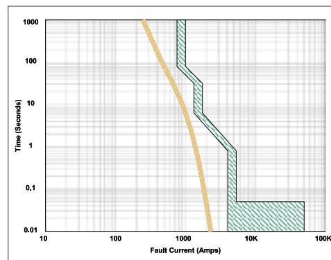
Figure 10 – Circuit Breaker Upstream of Fuse
