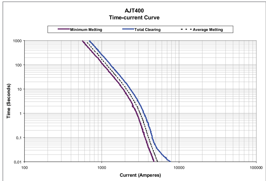
Figure 6 – Fuse Time-current Curves
