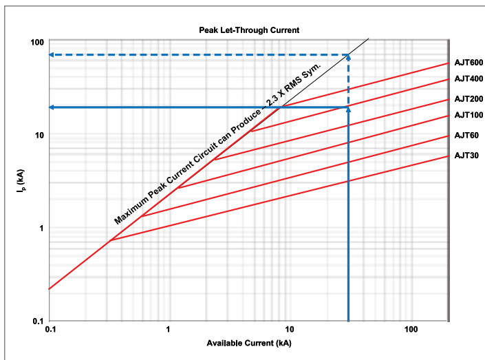
Figure 5 – Fuse Peak Let-Through Current Graph
