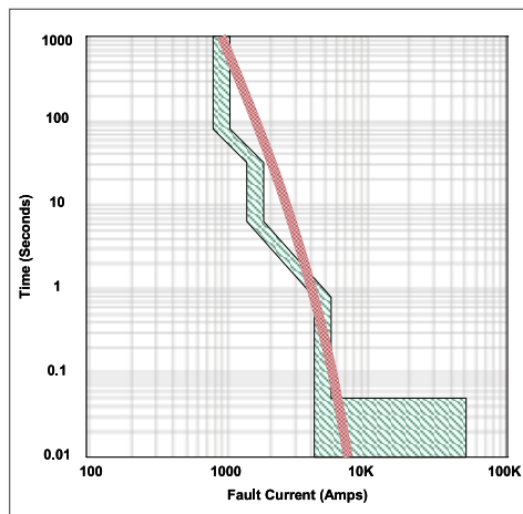
Figure 8 – Devices are not Selectively Coordinated
