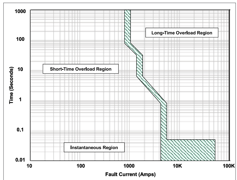
Figure 4 – Example of Circuit Breaker Time-current Curve
