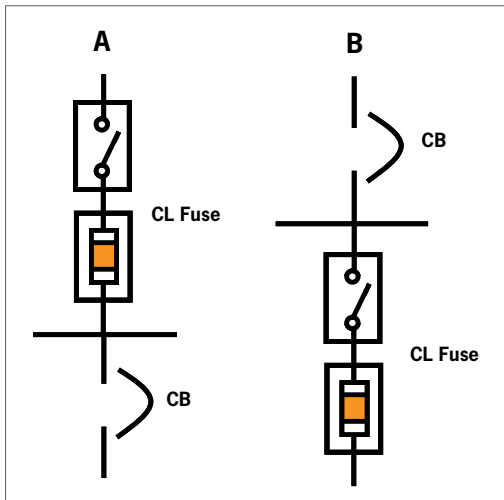
Figure 7 – Application A and B
