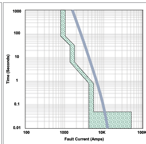
Figure 9 – Selectively Coordinated to 10kA
