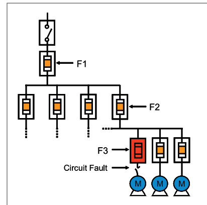
Figure 1 – Illustration of Selectively Coordinated System
