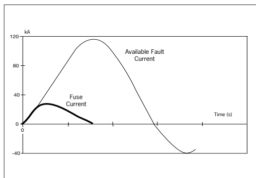
Figure 4. Fuse current limitation.
