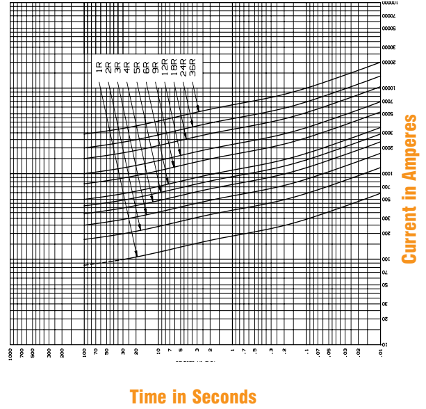
A240R, 2400 Volts
