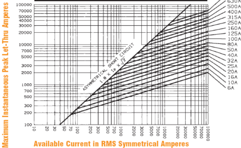
Peak Let-Through Current Data - 6-800 Amperes
