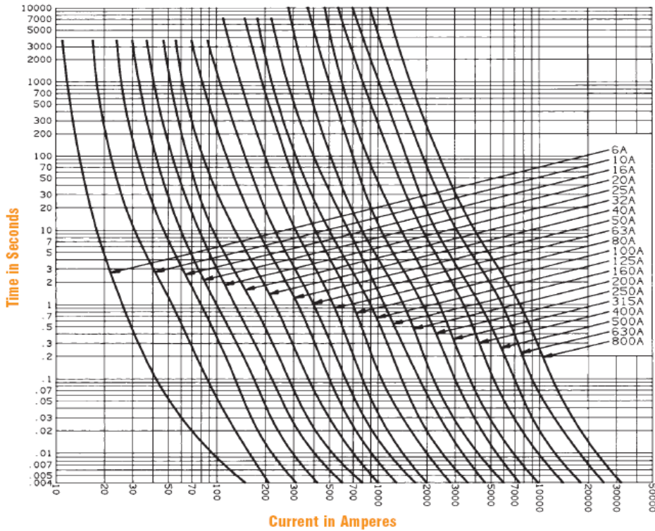
Melting Time - Current Data - 6-800 Amperes
