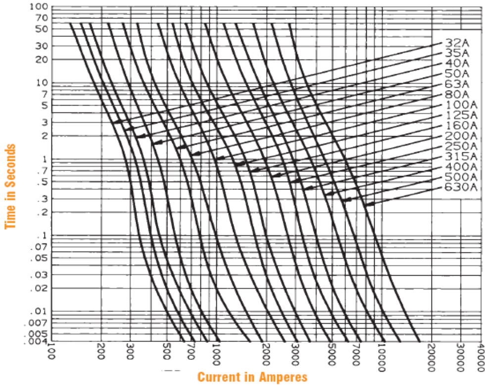
Melting Time - Current Data - 32-630 Amperes
