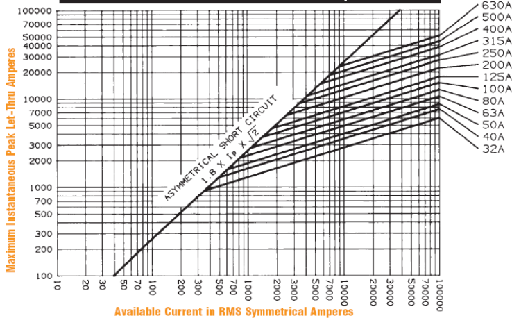
Peak Let-Thru Current Data - 32-630 Amperes
