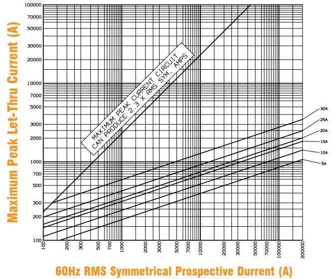
Peak Let-Thru Current
